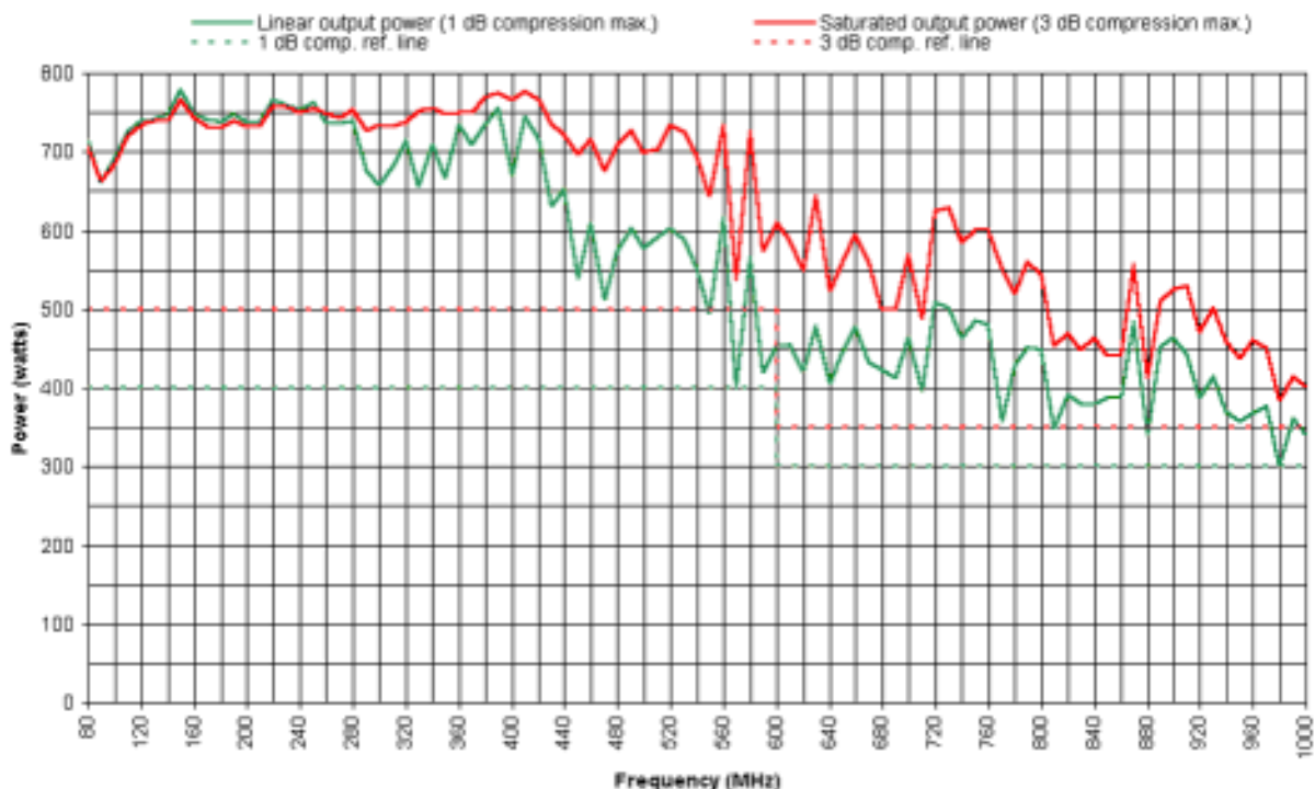
AP32 MT235 POWER AMPLIFIER - 80MHz - 1000MHz - Typical Power
