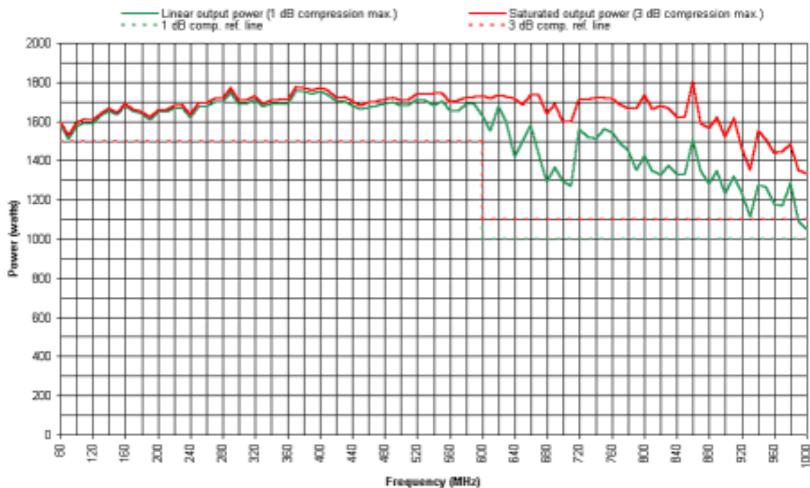
AP32 MT315 POWER AMPLIFIER - 80MHz - 1000MHz - Typical Power
